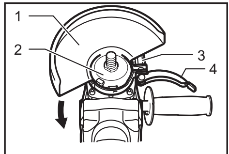
► 1. Wheel guard 2. Bearing box 3. Nut 4. Lever
